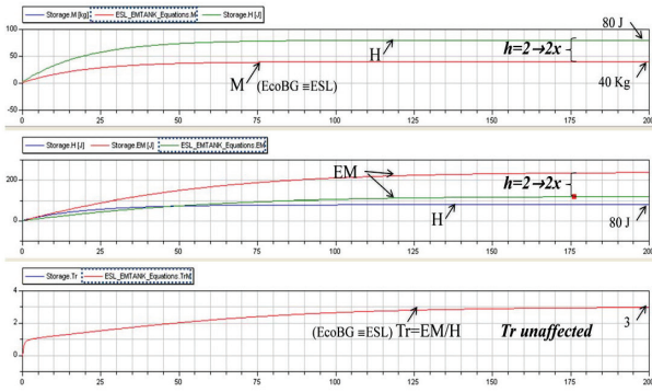
Figure 11: Scenario 1: Baseline with doubled specific enthalpy
