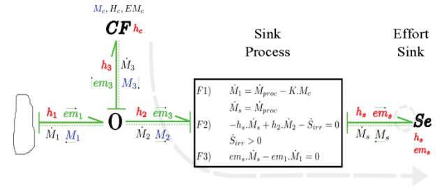
Figure 7: The Sink Process
