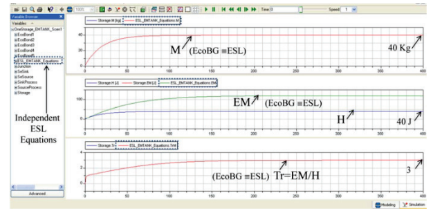
Figure 10: Baseline simulation of EMTANK with EcoBG and standard ESL equations. EcoBG mimics ESL results.
